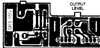
PCB-3 OUTPUT LEVEL & JACK P. C. BOARD HEADPHONES
